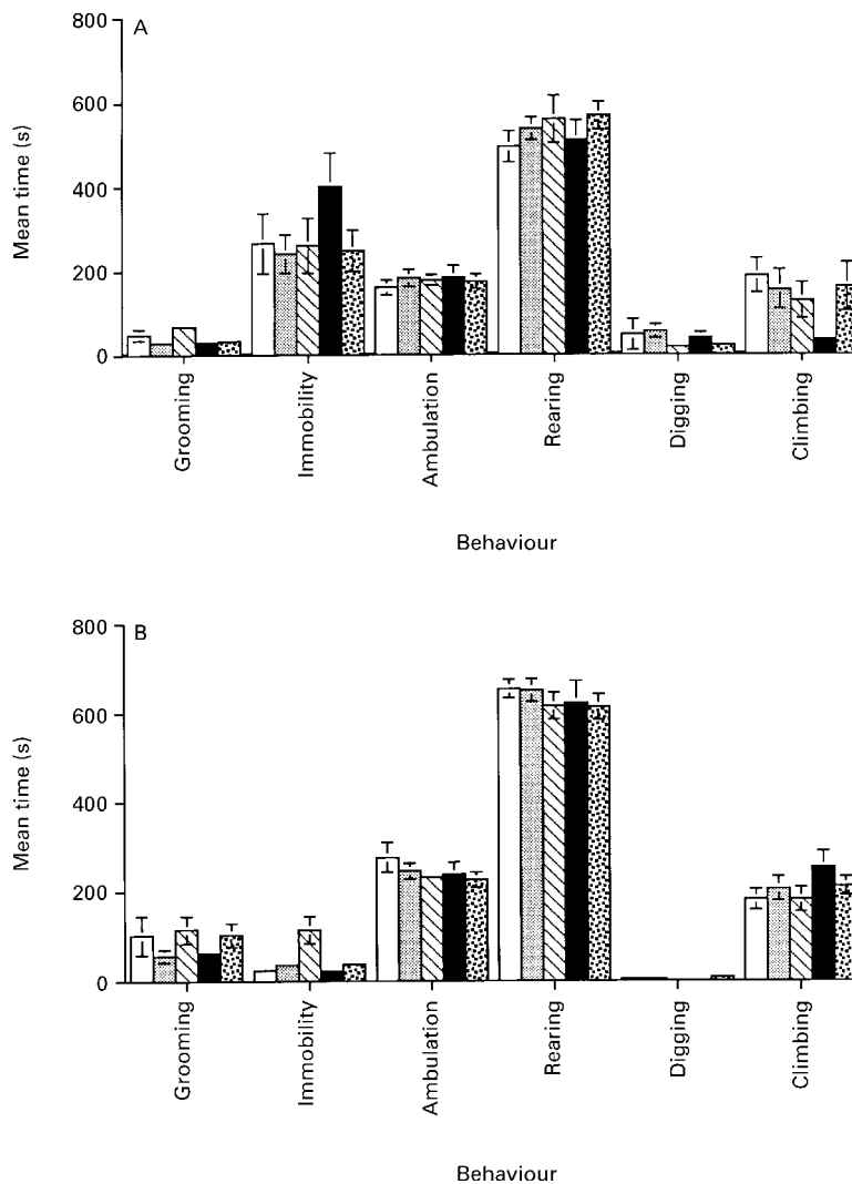
Fig. 1. The mean time ( \pm SE) spent at each murine behaviour pre-infection with Toxocara canis ova by LACA mice (A) and NIH mice (B). Dose group: \square , control; \text{▨} , 100; \text{▩} , 1000; \blacksquare , 3000; \text{▤} , trickle.
