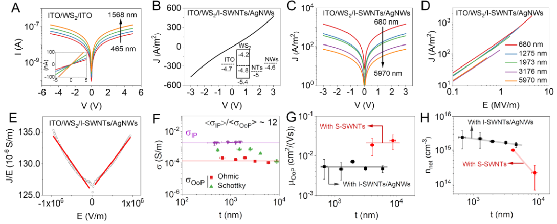
Figure 3. Electrical characterizations and properties of Ohmic devices. (A) Semi-log I - V curves of lateral ITO/WS 2 /ITO devices with various WS 2 thickness and inset is the linear I - V curves. (B) A representative J - V curve of an ITO/1.2 \mu\text{m} WS 2 /I-SWNTs/AgNWs device. (C) Semi-log J - V curves and (D) Log-Log J - E curves of ITO/WS 2 /I-SWNTs/AgNWs devices with various WS 2 thicknesses. (E) A typical J/E - E curve of an ITO/WS 2 /I-SWNTs/AgNWs device. (F) The in-plane and out-of-plane conductivity of WS 2 networks with Ohmic contacts plotted versus network thickness. In addition, the OoP conductivity estimated from the electrode limited devices is also shown. (G) and (H) show the WS 2 film thickness dependence of the OoP mobility \mu_{\text{OoP}} and carrier density n_{\text{net}} extracted either from I-SWNTs/AgNWs based or from S-SWNTs based devices, respectively. In F, G and H, the error bars represent averages over four independent devices per thickness.
