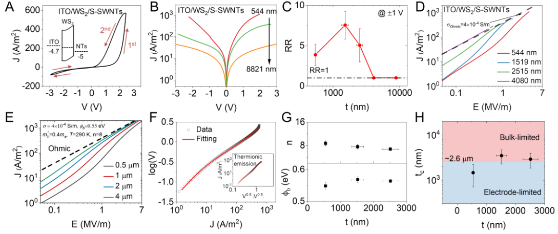
Figure 4. Electrical characterizations and properties of Schottky devices. (A) A typical J - V curve of ITO/ 1.5 \mu\text{m} \text{WS}_2 /S-SWNTs device after removing voltage drop on the S-SWNTs electrode. The inset in (A) is the band diagram of ITO, \text{WS}_2 , and S-SWNTs. (B) Semi-log J - V curves of ITO/ \text{WS}_2 /S-SWNTs devices with various \text{WS}_2 thicknesses. (C) Rectification ratio of ITO/ \text{WS}_2 /S-SWNTs devices at \pm 1 V for the second sweep. (D) J - E curves of ITO/ \text{WS}_2 /S-SWNTs devices with various \text{WS}_2 thicknesses. (E) Simulated J - E curves with various thicknesses. (F) A typical \log(V) - J curve of a Schottky device and its fitting curve. The inset in (F) is one typical J - V^{0.5} curve. (G) is extracted thickness-dependent ideality factor n (top) and potential barrier \phi_b (bottom), respectively. (H) is the plot of the transition film thickness t_c versus \text{WS}_2 film thickness. In C, G and H, the error bars represent averages over four independent devices per thickness.
