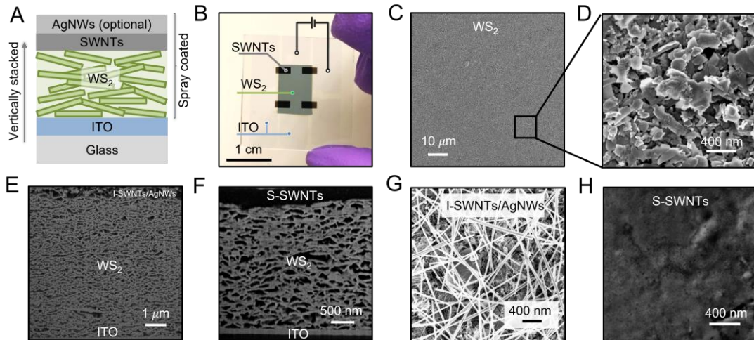
Figure 2. (A) Schematic diagram of the device structure and fabrication. (B) Photograph of ITO/WS 2 /S-SWNTs devices. Top-view SEM images of the spray coated WS 2 film (C), the WS 2 film with higher magnification (D). Cross-sectional SEM images of ITO/~6.5 μm WS 2 /I-SWNTs (E) and ITO/~2.5 μm WS 2 /S-SWNTs (F). Top-view SEM images of the double-layered I-SWNTs/AgNWs top electrode (G) and S-SWNTs electrode (H) on WS 2 film.
