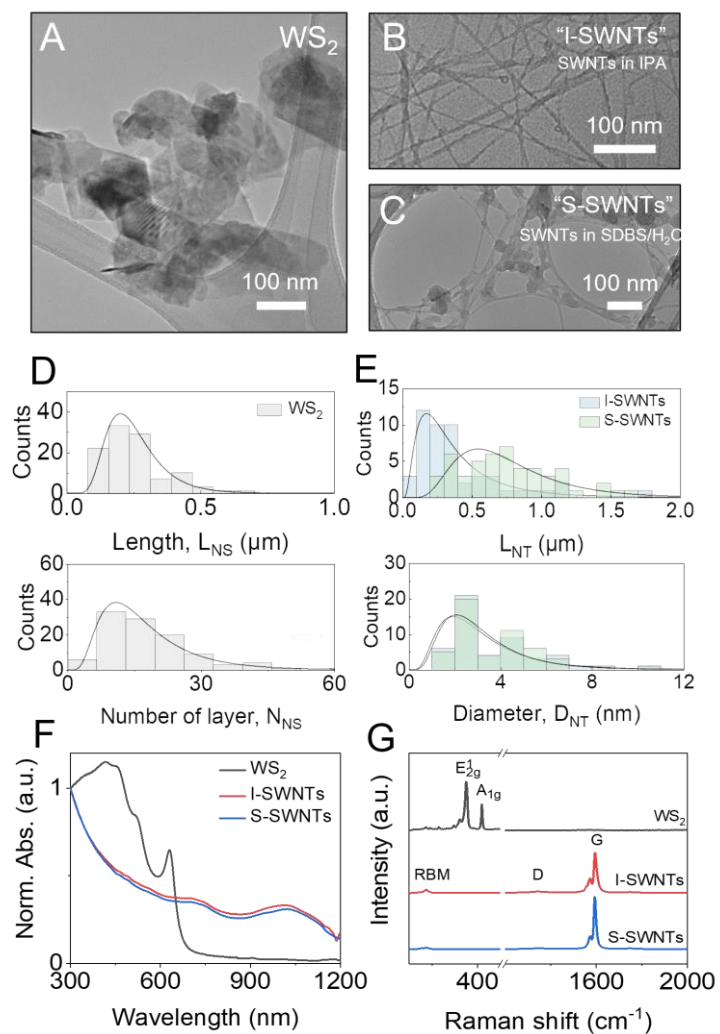
Figure 1. Basic characterizations of WS 2 nanosheets and SWNTs. TEM images of WS 2 nanosheets (A), I-SWNTs (B) and S-SWNTs (C). (D) Statistical analysis of the lateral length L_{NS} and the number of layer N_{NS} of WS 2 nanosheets extracted from AFM images. (E) Statistical analysis of the length L_{NT} and diameter D_{NT} of SWNTs extracted from AFM images. Normalized UV-Vis-NIR absorption spectra (F) and Raman spectra (G) of WS 2 , I-SWNTs and S-SWNTs.
