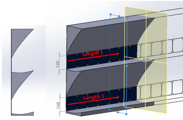
Figure 4. 4 System design inserted into Trace Pro
