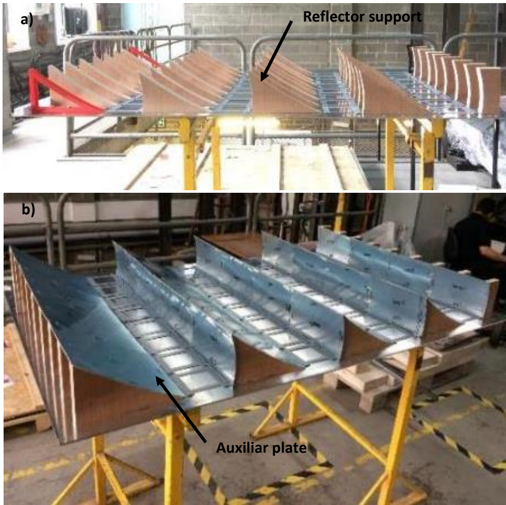
Figure 6. 15 (a) Reflector supports installed on the backplate (b) Final installation of the reflector supports with the auxiliary plate
