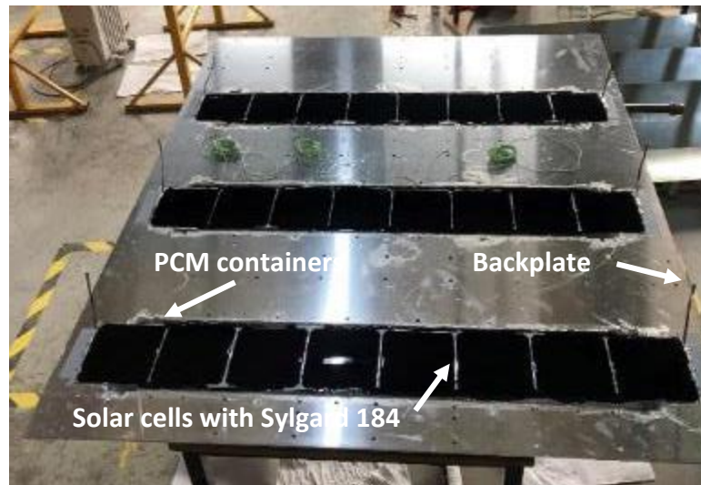
Figure 6. 28 CPC/PCM system with solar cells encapsulated
