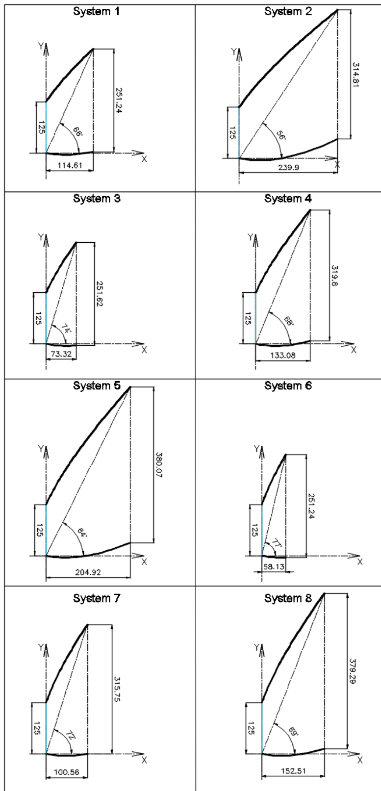
Figure 4. 14 Geometric characteristics of the CPC modelled for Ferrara
