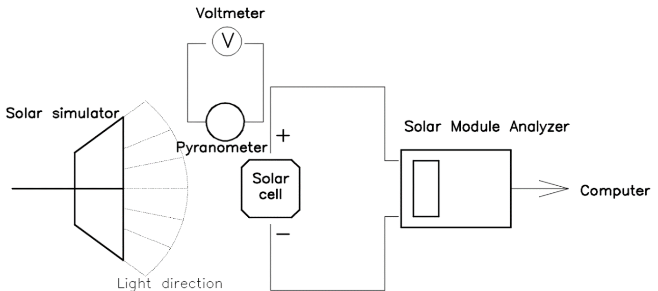
Figure 5. 13 Schematic diagram for SunPower characterization
