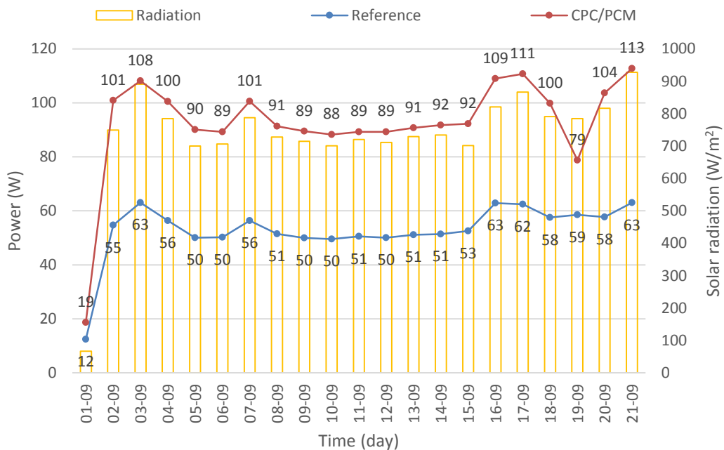
Figure 7. 8 Peak power output and solar radiation for CPC/PCM and Reference systems in September in Ferrara
