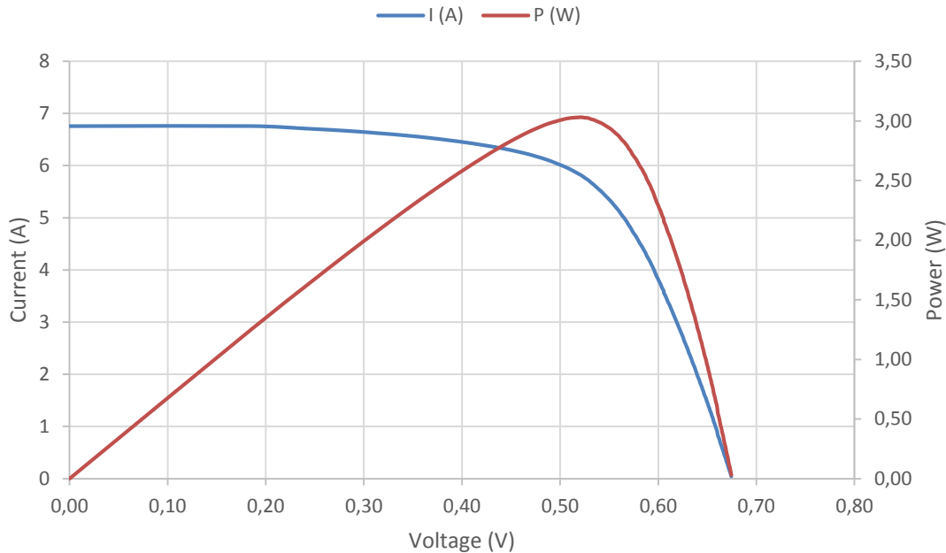
Figure 5. 15 IV Curve for a SunPower solar cell under 900 W/m 2
