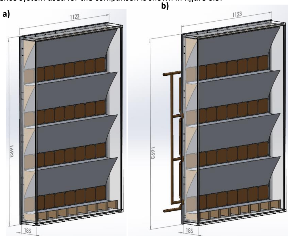
Figure 6. 4 CPC Systems designs for Ferrara (a) CPC system (b) CPC/PCM system
