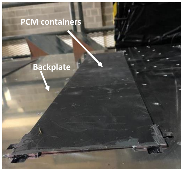
Figure 6. 27 CPC/PCM backplate with PCM containers fitting process
