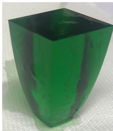
Figure 8. 3 Dielectric CPC printed using SL 3D printer
