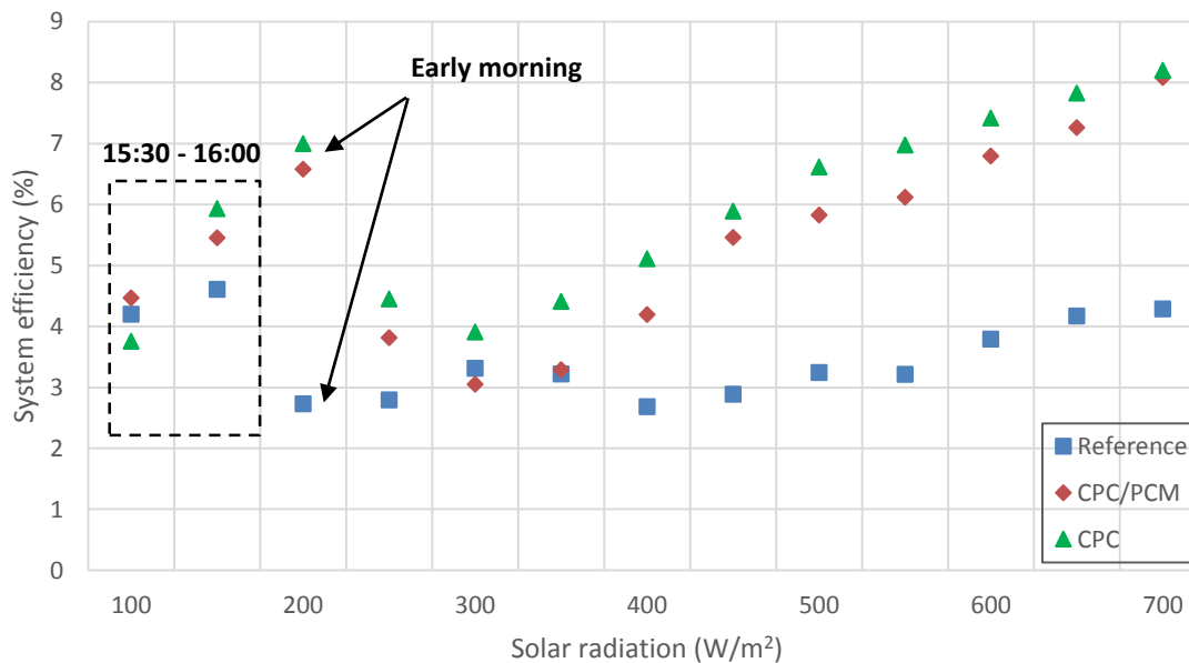
Figure 7. 35 Average system efficiency under clear sky for CPC, CPC/PCM and Reference systems
