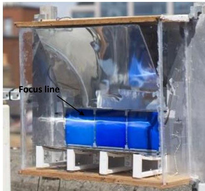
Figure 5. 20 Focus line on solar cells for small Ferrara prototype CPC system
