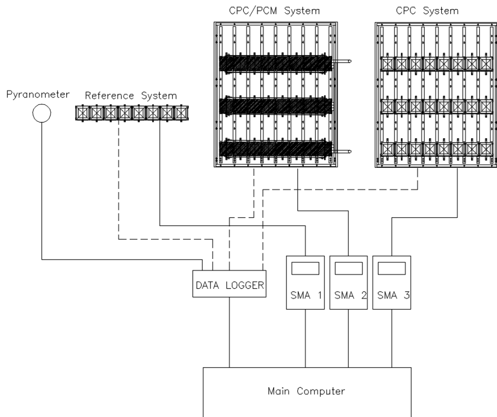
Figure 7. 20 Schematic monitoring connection for the CPC, CPC/PCM and Reference systems
