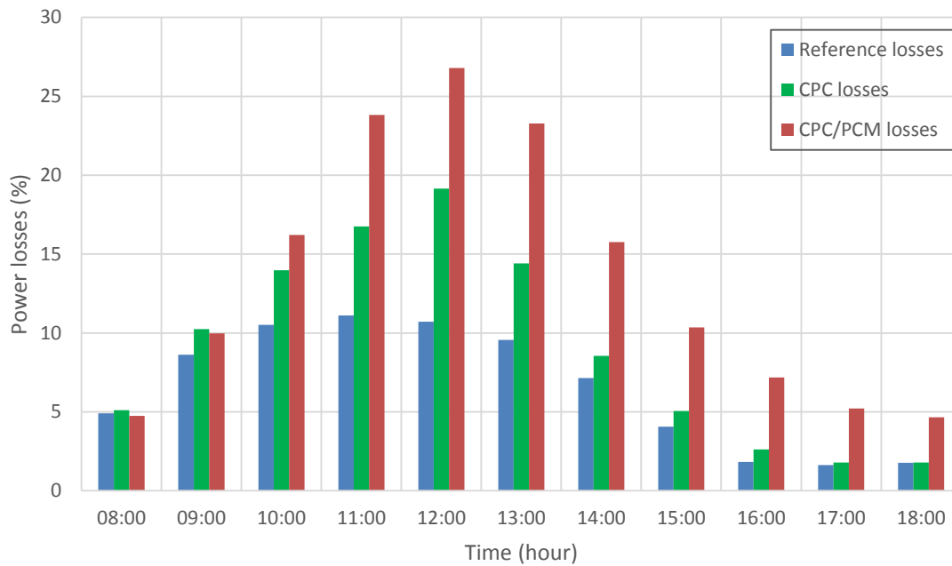
Figure 7. 44 Percentage power losses due to temperatures in the CPC, CPC/PCM and Reference systems under clear sky
