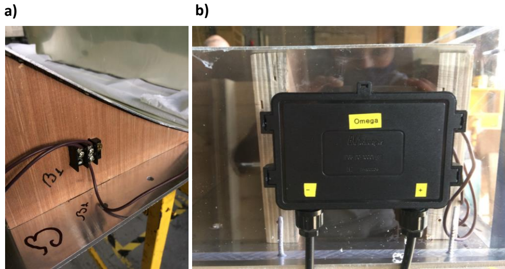
Figure 6. 18 (a) Internal connections between the solar cell strings and terminal block (b) Bypass diode box
