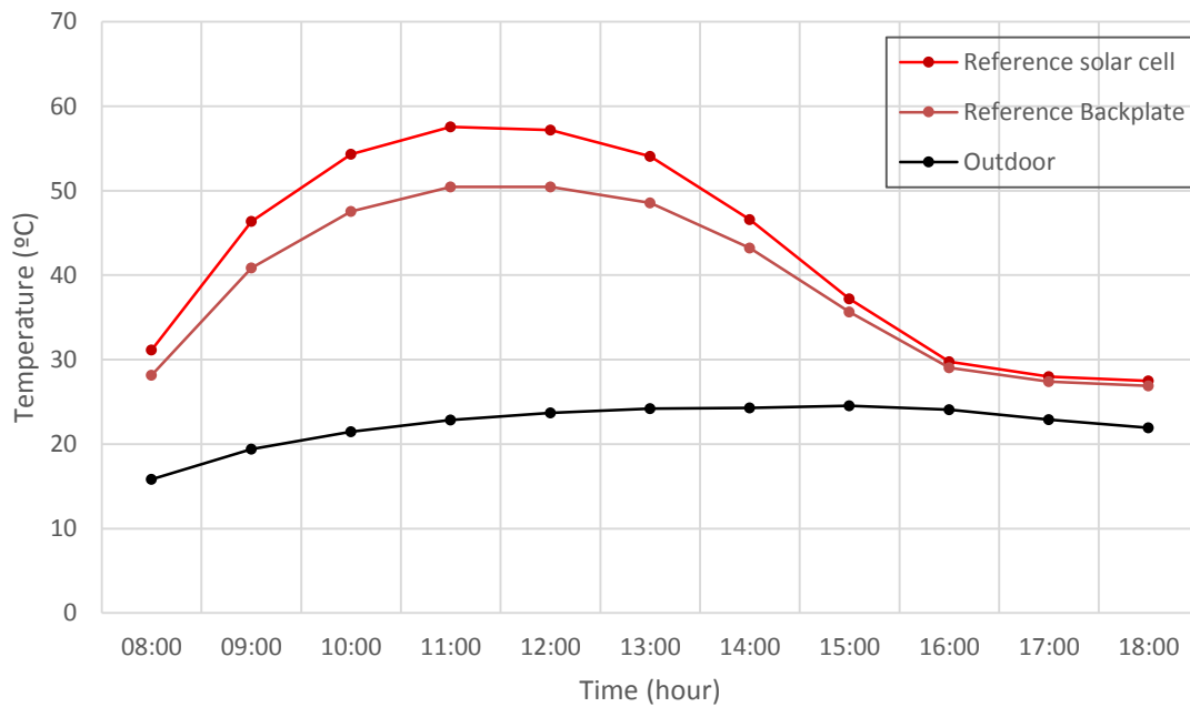
Figure 7. 40 Average temperature under clear sky on Reference system
