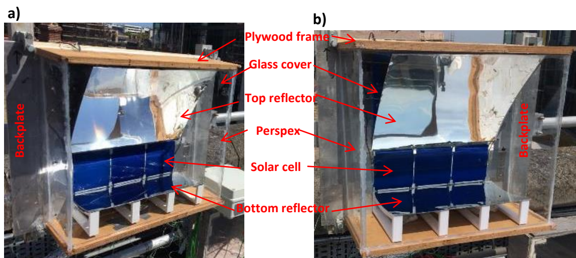
Figure 5. 18 Final assembly small prototypes CPC systems (a) Ferrara CPC system (b) Mayo CPC system
