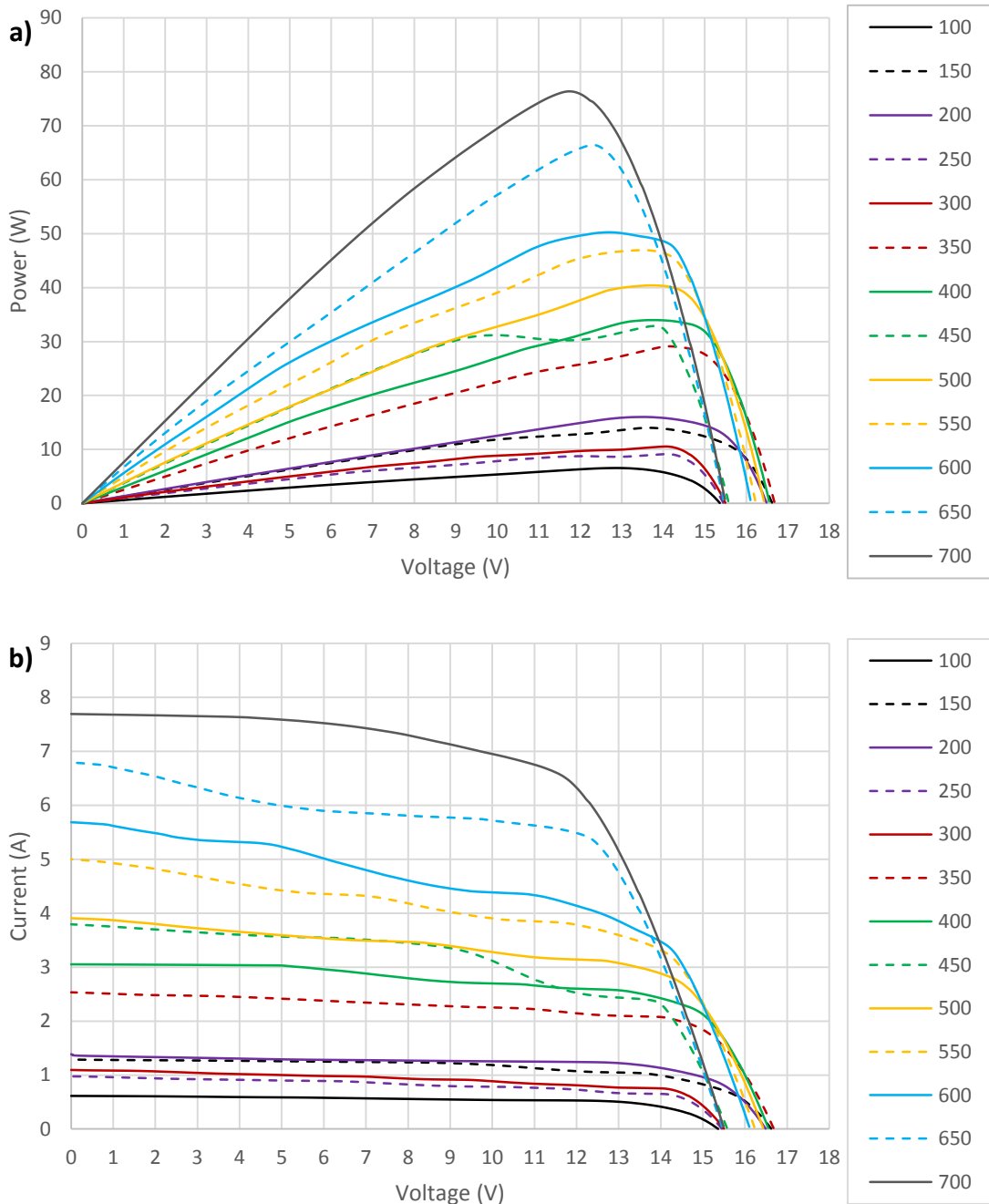
Figure 7.39 Maximum power output and I-V curve with solar radiation under clear sky of CPC system (a) Maximum power (b) I-V curve
