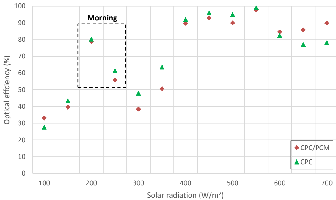
Figure 7. 34 Average optical efficiency under clear sky for CPC and CPC/PCM systems
