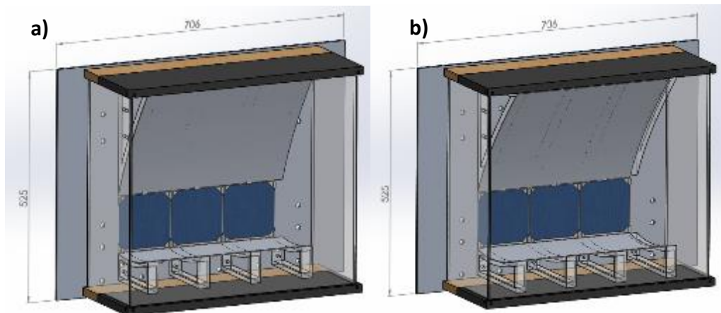
Figure 5. 1 Design CPC system small prototypes (a) CPC system Ferrara (b) CPC system Mayo
