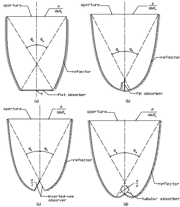
Figure 2. 2 Different CPC configurations (Mallick, 2003) (a) CPC with flat absorber, (b) CPC with fin, (c) CPC with “inverted vee” absorber, (d) CPC with tubular absorber
