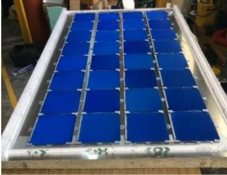
Figure 6. 22 PV Reference System fully assembled
