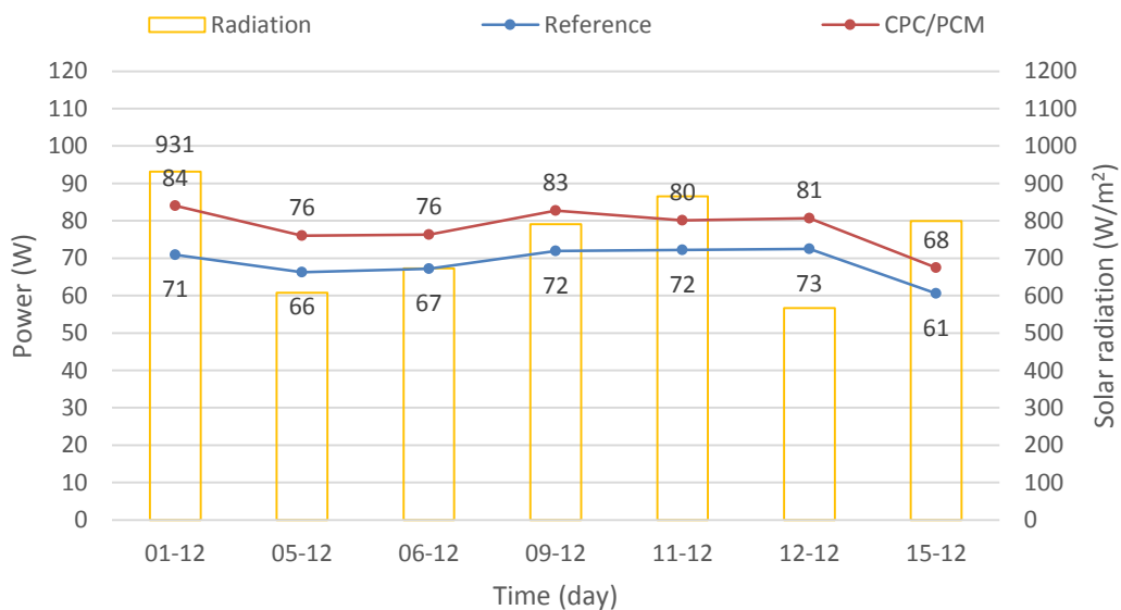
Figure 7. 17 Peak power output and solar radiation for CPC/PCM and Reference systems in December in Ferrara
