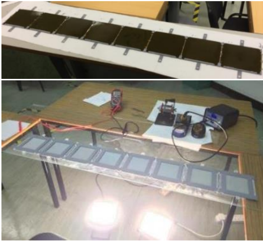
Figure 3. 11 Connection table with halogen lamps
