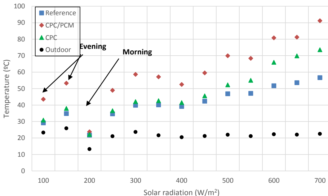
Figure 7. 30 Average solar cell temperature under clear sky for CPC, CPC/PCM and Reference systems
