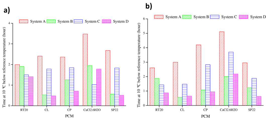
Figure 2. 15 Results from experiments at (a) 750 \text{ W/m}^2 and (b) 1000 \text{ W/m}^2 (Hasan, 2010)
