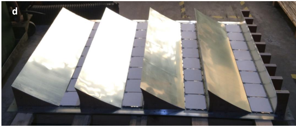
Figure 6. 16 Alanod reflector gluing process
