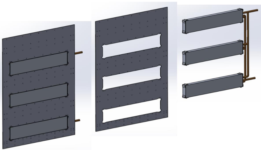
Figure 6. 24 Schematic design of the backplate corresponding to CPC/PCM system for Mayo
