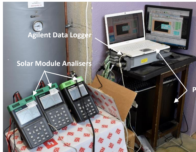
Figure 7. 19 Monitoring system used in the characterization of the CPC, CPC/PCM and Reference systems
