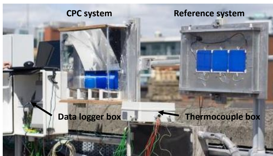
Figure 5. 19 Small Ferrara prototype CPC system and Reference system installed on the roof
