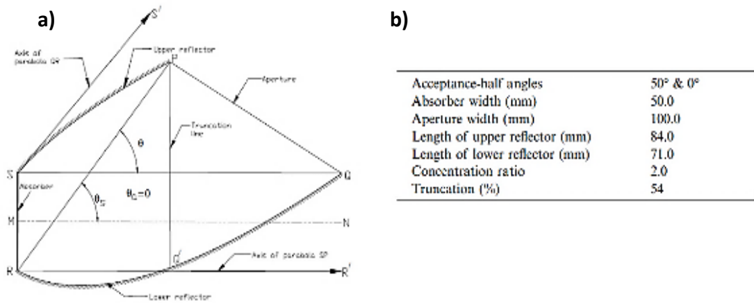
Figure 2. 5 Asymmetric compound parabolic concentrator for building integration in the UK with acceptance-half angles of 0 ° and 50 ° (Mallick et al., 2004)
