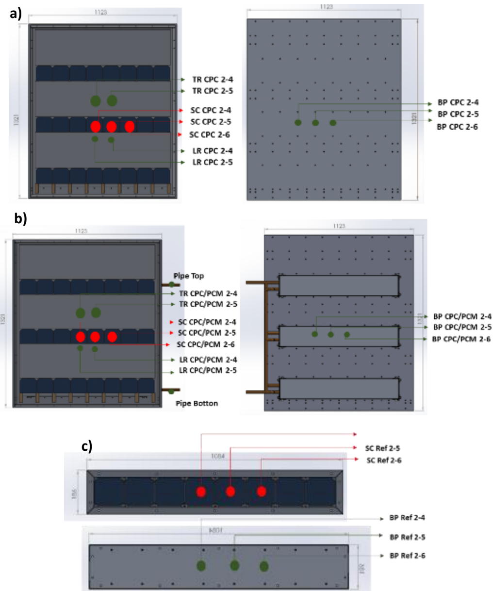
Figure 6.30 (a) Thermocouples location for CPC system (b) CPC/PCM system (c) Reference system
