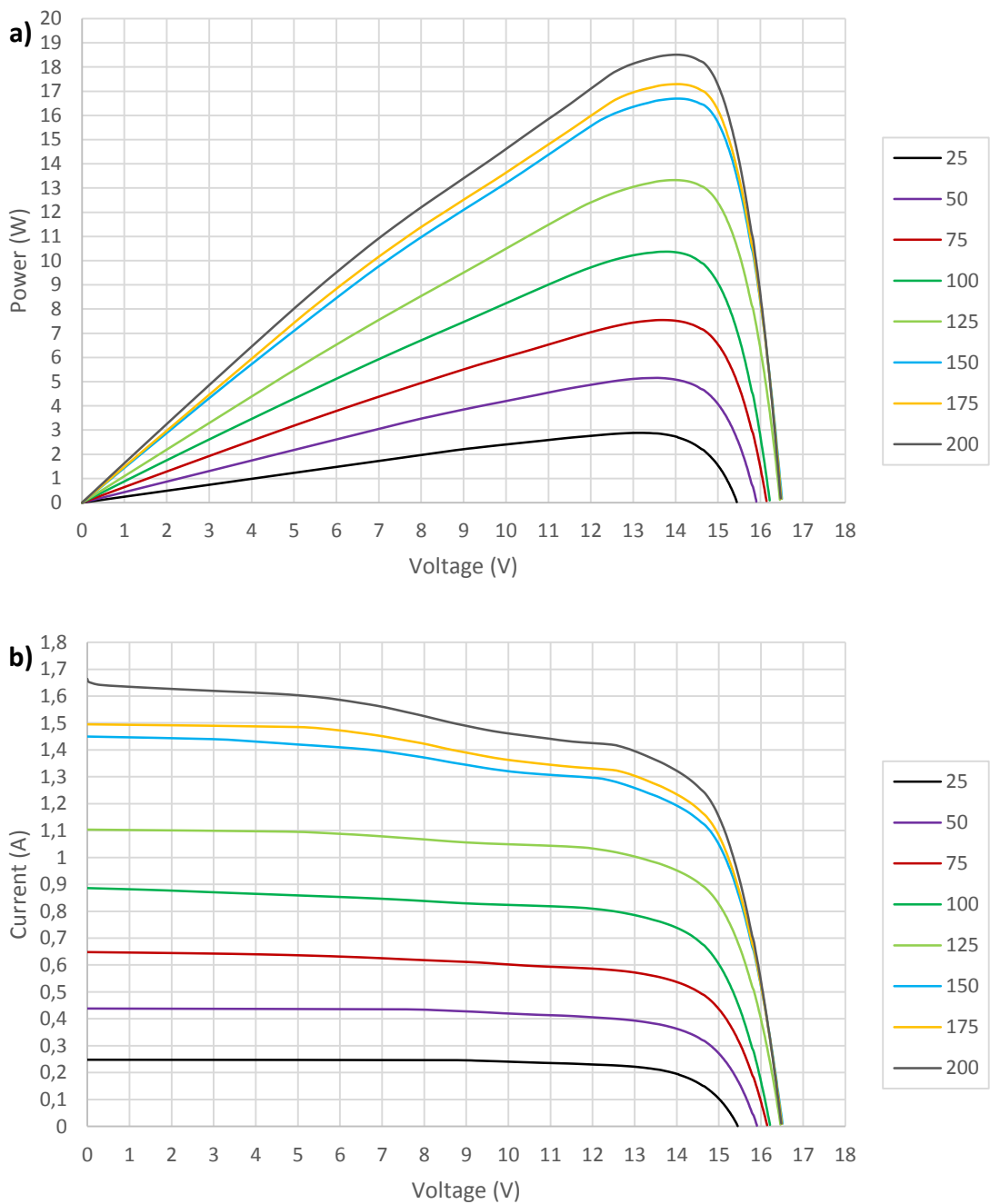
Figure 7. 63 Maximum power output and I-V curve with diffuse solar radiation of CPC/PCM system (a) Maximum power (b) I-V curve
