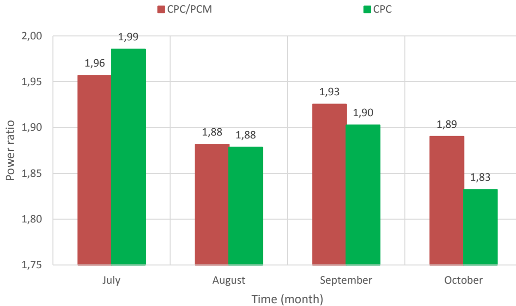
Figure 7. 72 Average power ratio for four months for CPC and CPC/PCM systems
