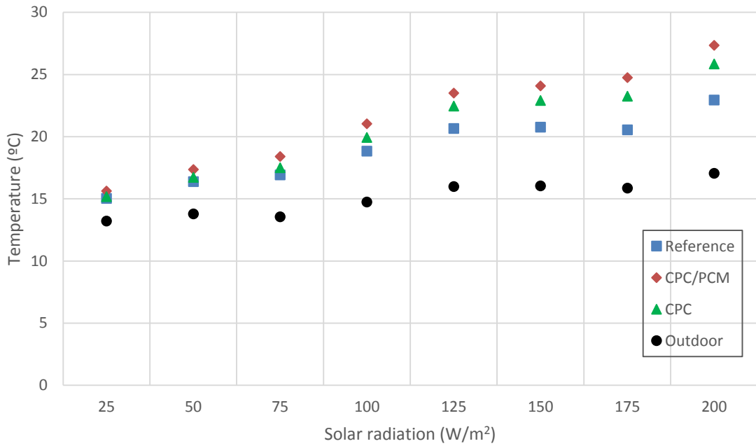
Figure 7. 55 Average solar cell temperature with diffuse solar radiation for CPC, CPC/PCM and Reference systems
