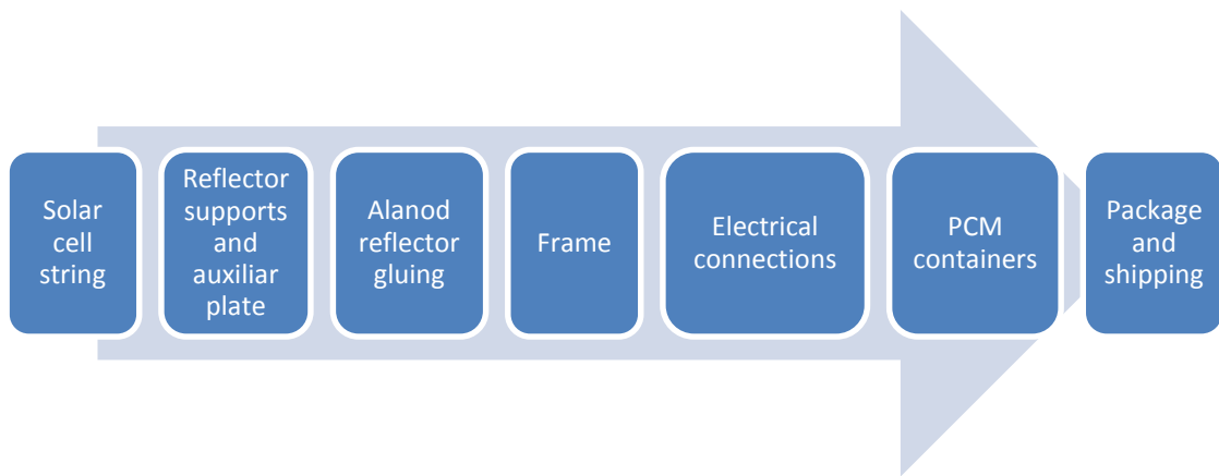
Figure 6. 13 Assembly process flow chart for Ferrara systems
