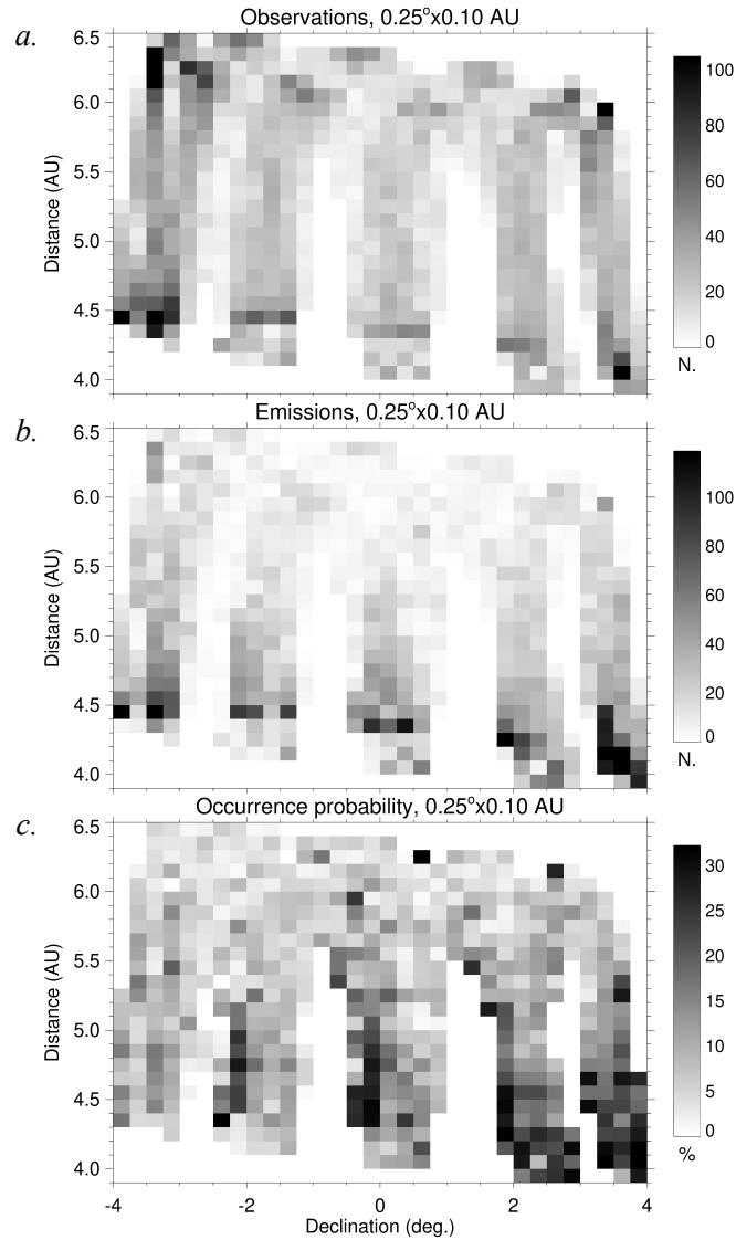
Figure 4: Distributions of all the observations of Jupiter ( a ) by the Nançay Decameter Array, from 1978 to 2020; of all the detected Jovian DAM emissions ( b ); and of the emissions' occurrence probability ( c ), as a function of the jovicentric declination of the Earth and of the Earth-Jupiter distance.
