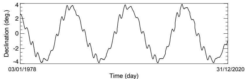
Figure 2: Daily variation of the Jovicentric declination of the Earth, from Jan. 3th, 1978 to Dec. 31st, 2020.
