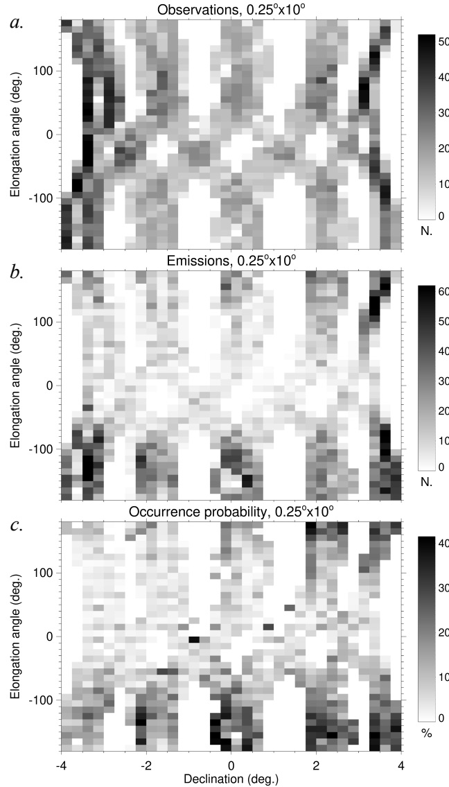
Figure 5: Distributions of all the observations of Jupiter (a) by the Nançay Decameter Array, from 1978 to 2020; of all the detected Jovian DAM emissions (b); and of the emissions' occurrence probability (c), as a function of the jovicentric declination of the Earth and of Jupiter's elongation.
