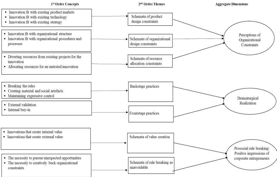
Figure 1. Data structure
