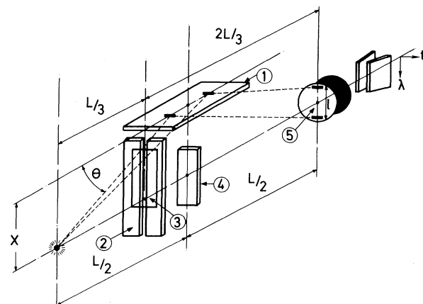
FIG. 1. Experimental arrangement for recording streaked spectra: (1) crystal of thallium-acid-phthalate (TIAP) or pentaerythritol (PET), (2) adjustable entrance slit, (3) beryllium filter, (4) baffle, and (5) CsI photocathode.
