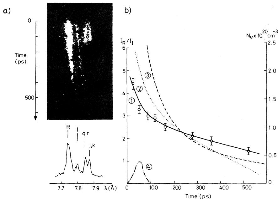
FIG. 2. (a) Streaked spectrum from a plane aluminum target with a densitometer trace at t = 50 ps showing the Al XII 1^1S_0-2^1P_1 resonance line ( R ), its associated dielectronic satellites ( q, r, j, k ), and the 1^1S_0-2^3P_1 intercombination line ( I ), recorded with a gold photocathode. (b) Experimental and calculated data showing the time variation of (1) the measured intensity ratio I_R/I_I of resonance-to-intercombination line, (2) the electron density N_e from (1) above, (3) N_e for self-similar planar expansion fitted at t = 250 ps, and (4) the laser pulse.
