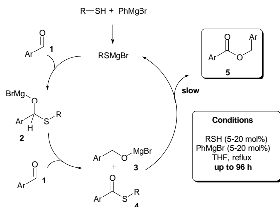
Figure 1. The thiolate catalysed homo-Tishchenko reaction
