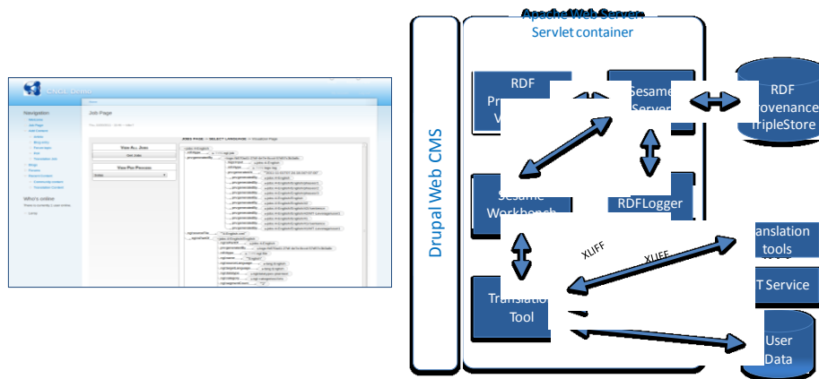
Fig. 2. CMS-Localisation System architecture with provenance visualiser screenshot
