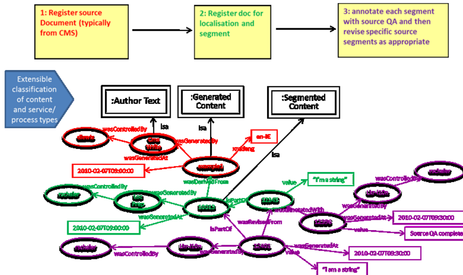
Fig. 1. Example of RDF provenance capture for a three step workflow
