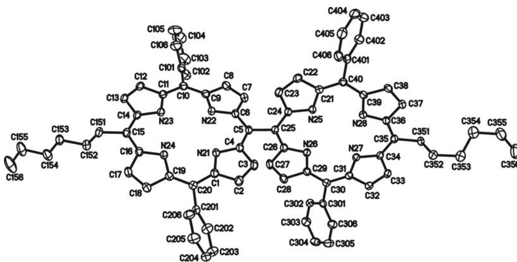
Fig. 1. View of the molecular structure of 6 in the crystal. Displacement ellipsoids are drawn at the 50 % probability level. Hydrogen atoms have been omitted for clarity.
