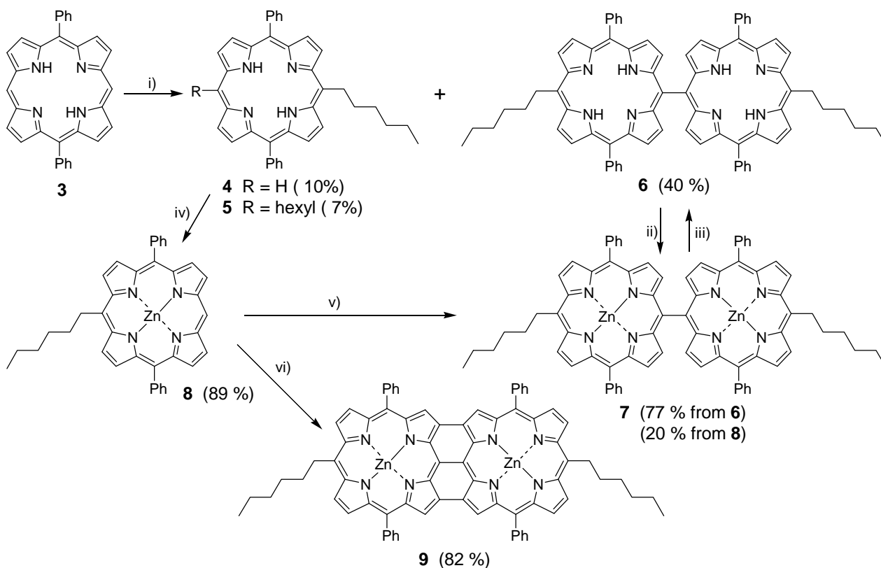
Scheme 1. Synthesis of meso-meso-linked bisporphyrins. i) n HexLi, DDQ, THF -78 °C; ii) Zn(II)(OAc) 2 , CH 3 OH, CH 2 Cl 2 , 20 °C; iii) Sc(OTf) 3 , DDQ, toluene, Δ; iv) ZnO, TFA, CH 2 Cl 2 ; v) Sc(OTf) 3 , DDQ, toluene, Δ; vi) Sc(OTf) 3 , DDQ, toluene, 20 °C.
