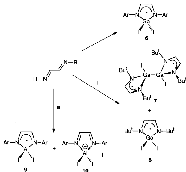
Scheme 1 Reagents and conditions: i, GaI, toluene, R = Ar; ii, GaI, toluene, R = Bu t ; iii, AlI 3 /Al, toluene, R = Ar.
