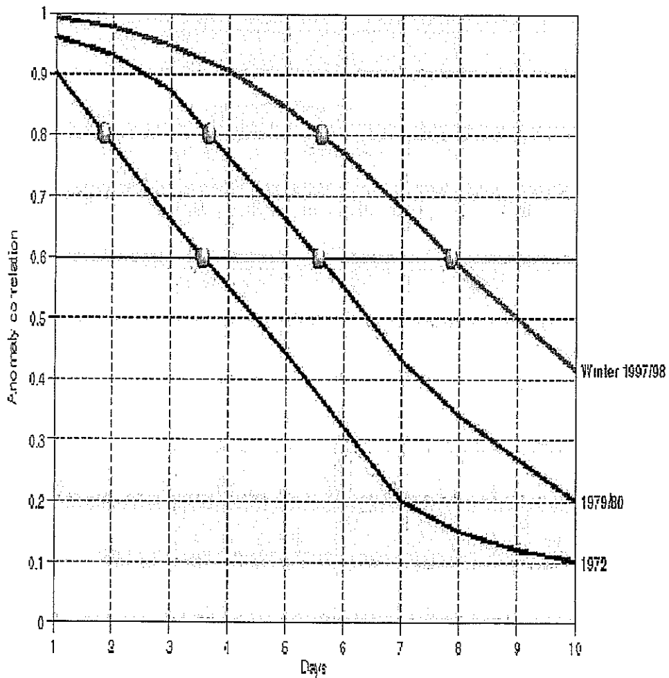
Northern Hemisphere (DJF) Anomaly correlation 500 hPa
