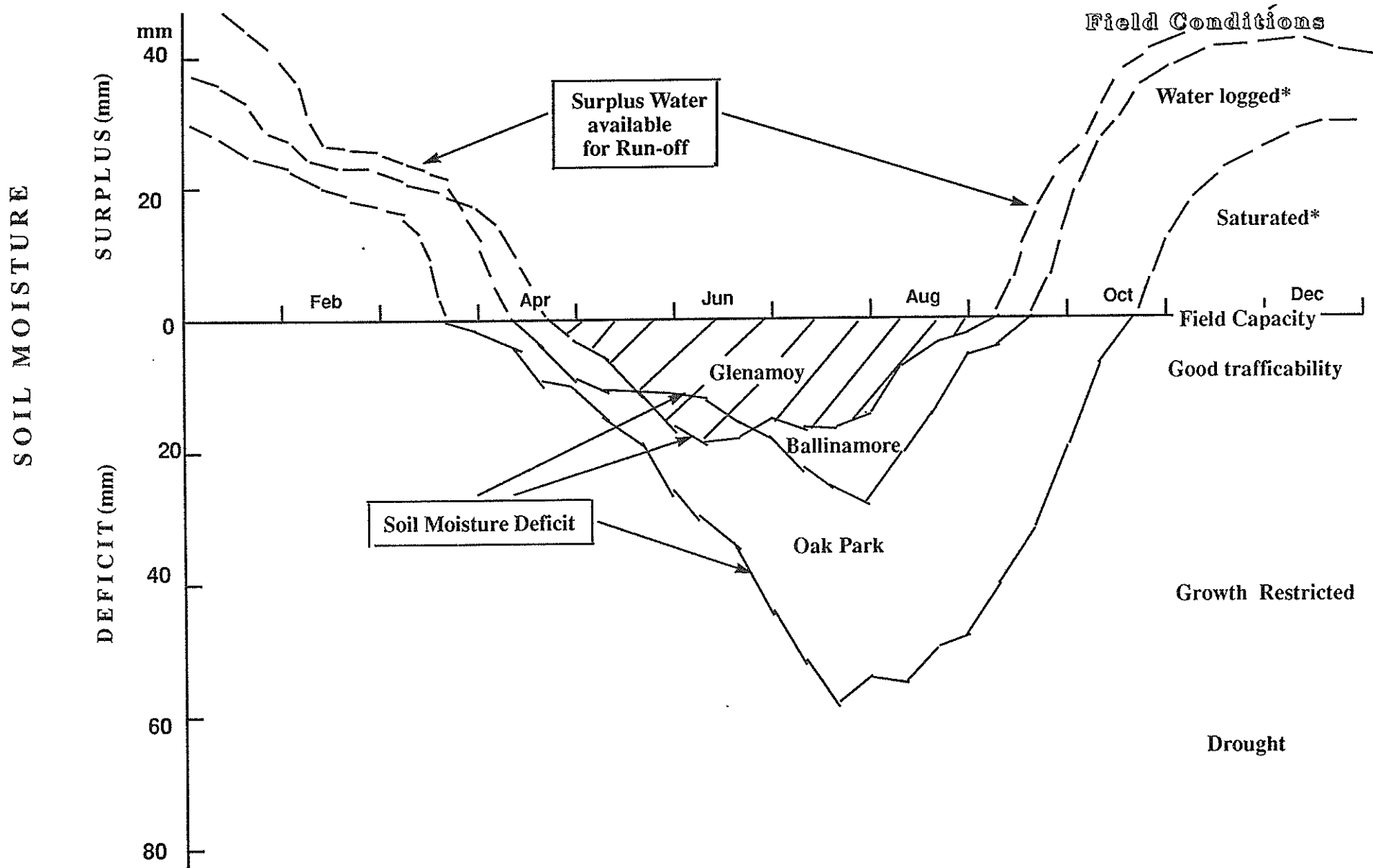
Run-off water (10-day totals) and Soil Moisture Deficit at Glenamoy, Ballinamore and Oak Park — median values (mm) for period 1971-1987 * These conditions depend on the drainage characteristics of soil
