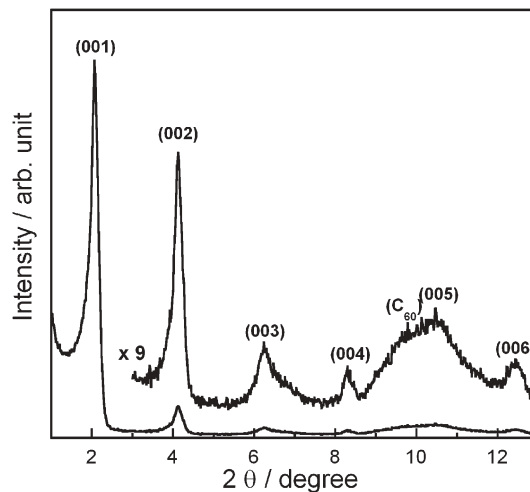
Fig. 3 X-ray diffraction diagram of a cast film of 1 .
