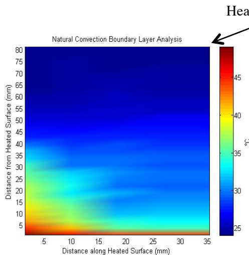
Figure 12. Thermal boundary layer analysis of the multiple orifice heat sink from natural convection
