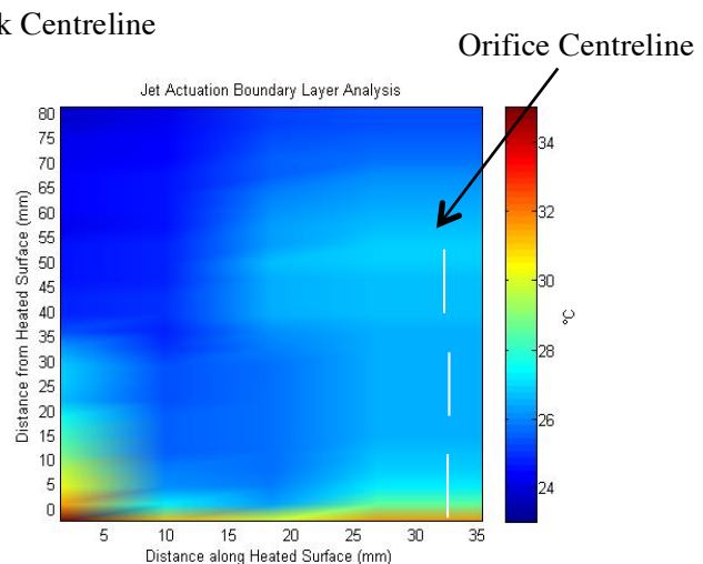
Figure 13. Thermal boundary layer analysis of the multiple orifice heat sink from jet actuation
