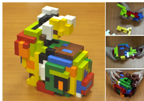
Fig. 6. An example interlocking puzzle with LEGO bricks, from [26].
