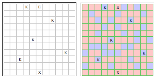
Fig. 9. Example of a chess maze for a rook from [27]; E represents the entry tile, X the exit tile, and the K tiles have knights on them. The left image is what appears to the player, the right image has the obstructed squares marked in blue.
