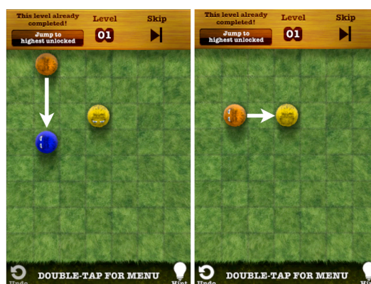
Fig. 3. Sample moves on a Fling! (2013) board, from [20].
